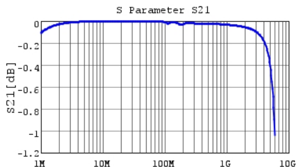
GRM3195C1H103JA01 S21 DCOV, 25degC
