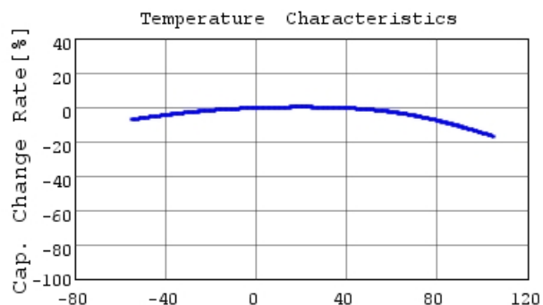
■ GRT033C80J223KE01 C-Temp. capchange, DC0.0V,
