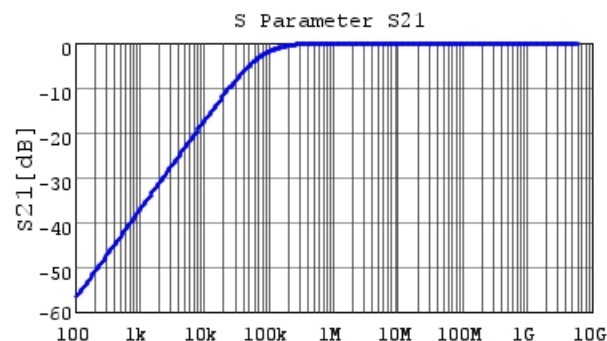
■ GRT033C80J223KE01 S21 DC0V, 25degC
