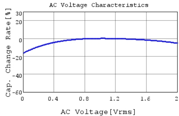
GRT155C80J475ME13 C-AC Voltage capchange, D
