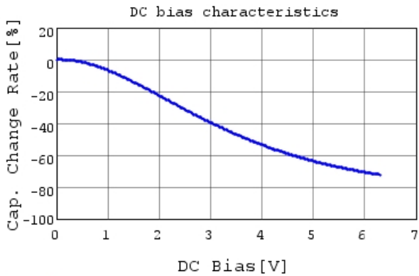
GRT155C80J475ME13 C-DC bias capchange, 25.0C
