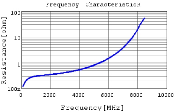
GRT1885C2A7R0DA02 R DCOV, 25degC
