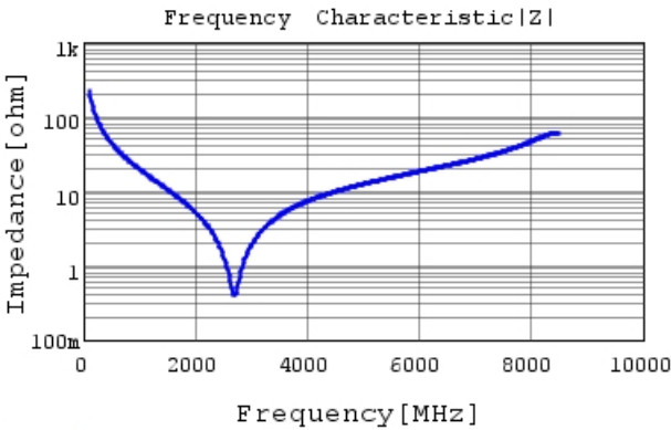
GRT1885C2A7R0DA02 |Z| DCOV, 25degC
