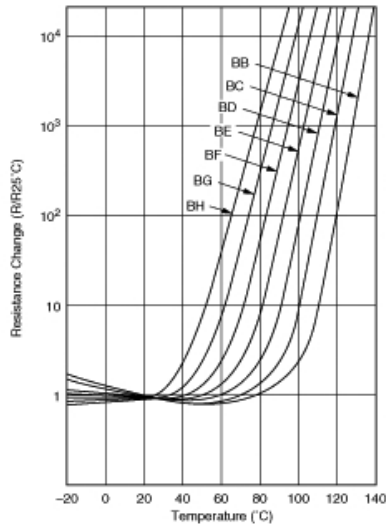
Resistance-Temperature Characteristics
