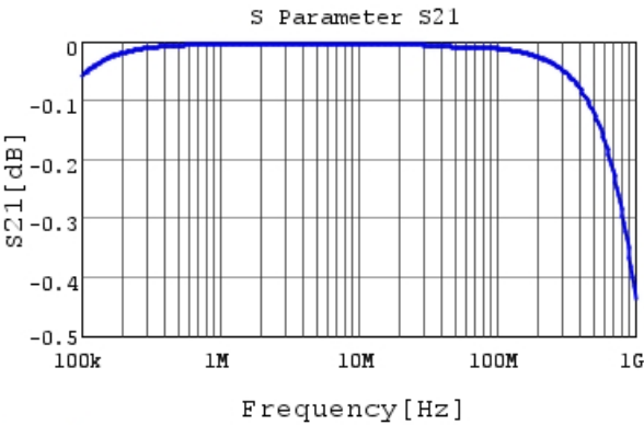
RHEL81H154K1K1H03B S21 DCOV, 25degC
