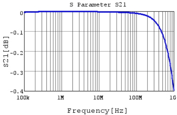
RHEL81H684K2A2H03B S21 DCOV, 25degC
