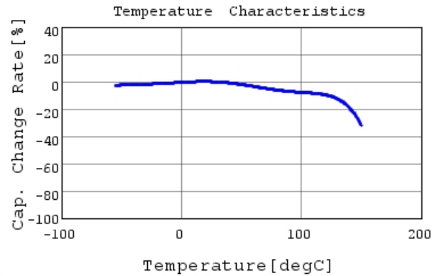
RHEL81H684K2A2H03B C-Temp. capchange, DCOV,
