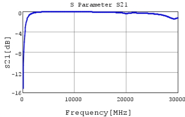
GRM0225C1H2R8WA03 S21 DCOV, 25degC
