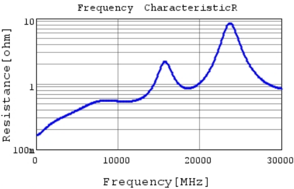
GRM0225C1H4R2CA03 R DCOV,25degC
