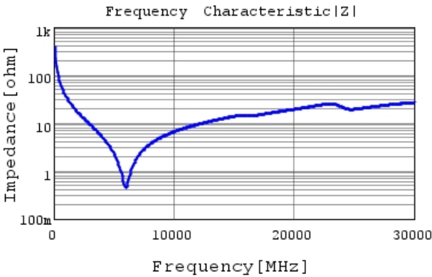
GRM0225C1H4R2CA03 |Z| DCOV,25degC
