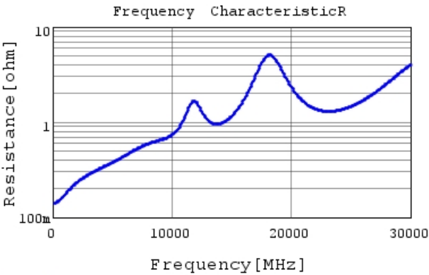
GRM0225C1H7R6WA03 R DCOV,25degC
