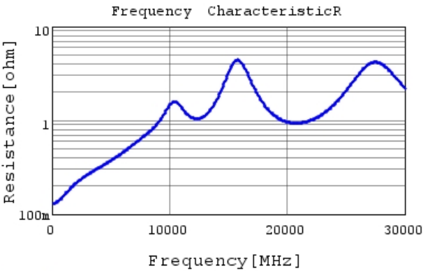
GRM0225C1H9R6WA03 R DCOV, 25degC
