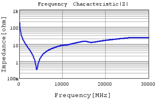
GRM0225C1H9R6WA03 |Z| DCOV, 25degC
