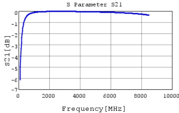
GRM0332C2A9R0CA01 S21 DCOV, 20degC
