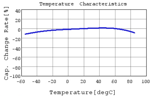
GRT033R60J105ME13 C-Temp. capchange, DC0.0V,
