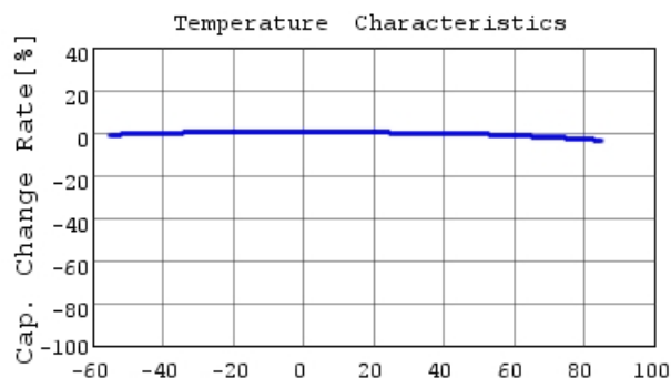
Temperature [degC] GRT033R61E221KE01 C-Temp. capchange, DC0.0V,
