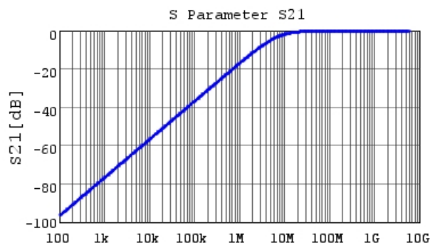
Frequency [Hz] GRT033R61E221KE01 S21 DC0V, 25degC
