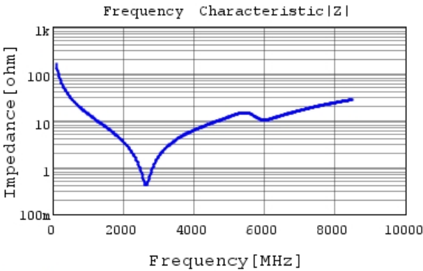
GRT1555C1H100JA02 |Z| DCOV,25degC
