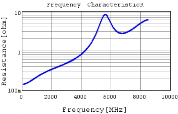
GRT1555C1H100JA02 R DCOV,25degC
