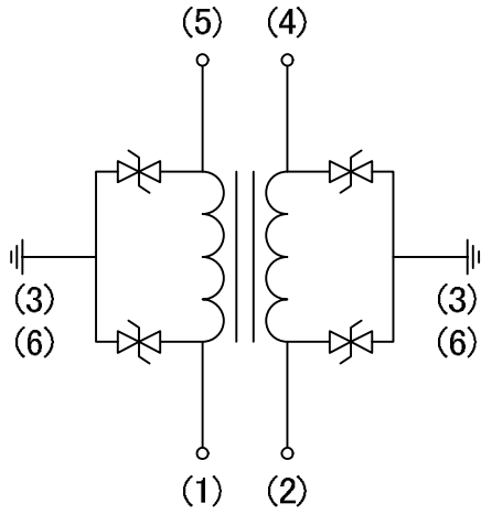
LXES11D series / LXES0ND series
