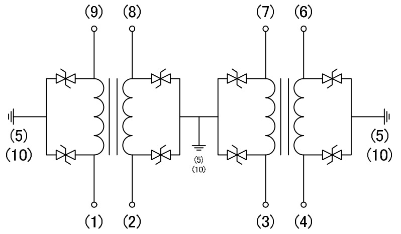
LXES21D series/ LXES18D series
