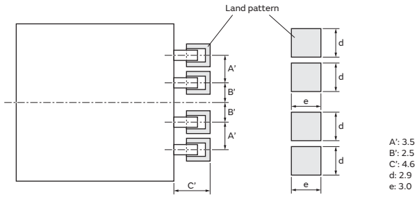
Fig. Land pattern and Product package
