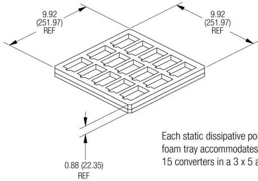
BASEPLATE VERSION
