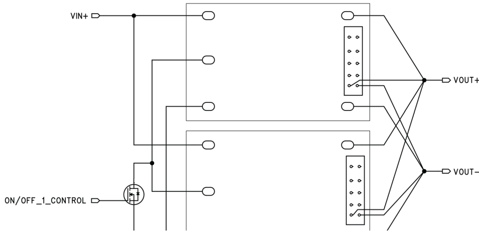
Figure 3. Load Sharing Block Diagram
