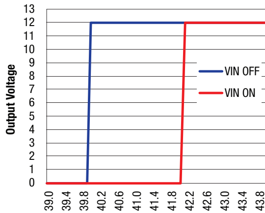
Output v. Input Voltage @ Full Load
