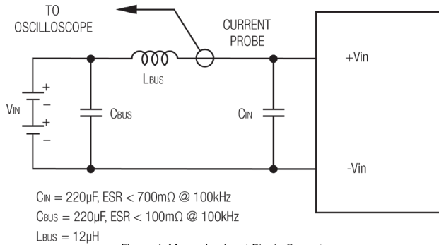
Figure 4. Measuring Input Ripple Current
