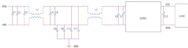
Figure 7. Conducted Emissions Test Circuit
