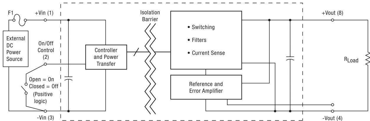
Figure 1. Connection Diagram (without digital interface) Typical topology is shown. Murata Power Solutions recommends an external fuse.
