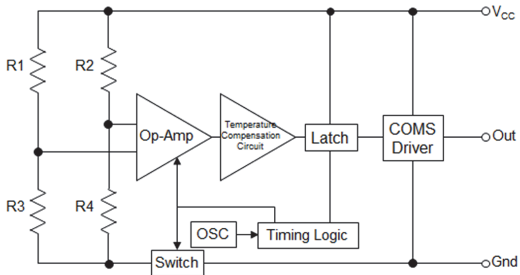
The intermittent switch circuit inside R1-R4:MR Elements
