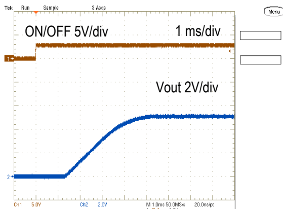
On/Off Enable Delay (Vin=12V, Vout=5.0V, Iout=6A, Cload=400uF)
