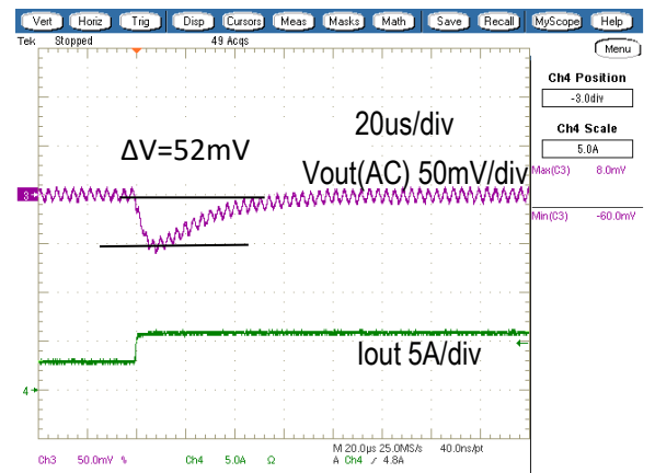
Step Load Transient Response (Vin=12V, Vout=3.3V, Cload=400uF, Iout=3A to 6A, 2.5A/us)
