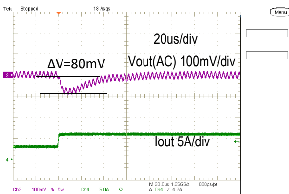
Step Load Transient Response (Vin=12V, Vout=5.0V, Cload=400uF, Iout=3A to 6A, 2.5A/us)
